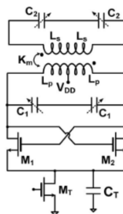
Figure 1: Schematic of a class-F oscillator [1]
